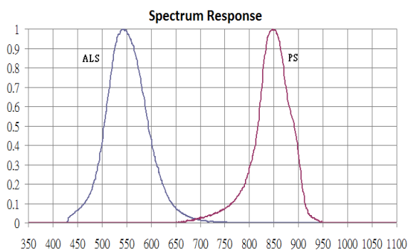
Fig.7 Spectrum Response
